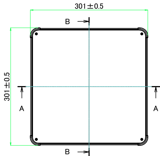
A view
